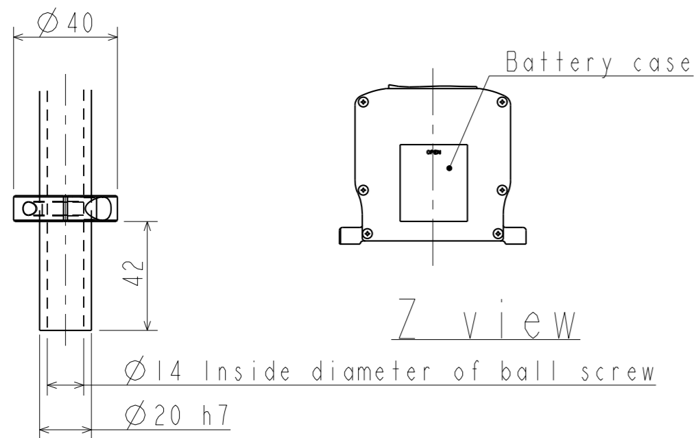
Detail installation view of hand Scale 1:2
