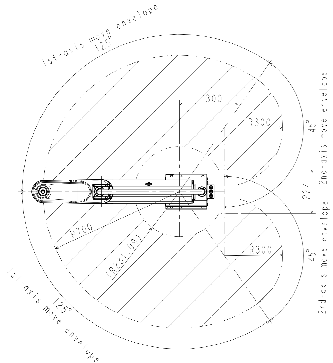
Move envelope Scale 1:10
