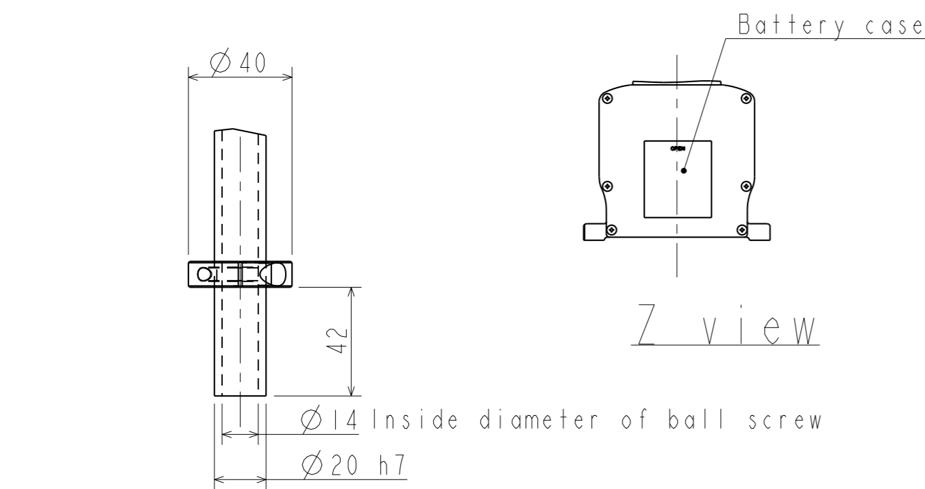
Detail installation view of hand Scale 1:2
